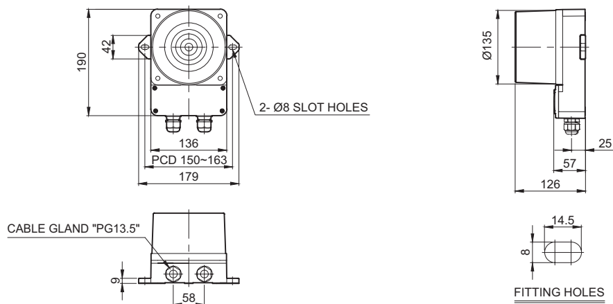
QWH35T/ QWH35TSD
