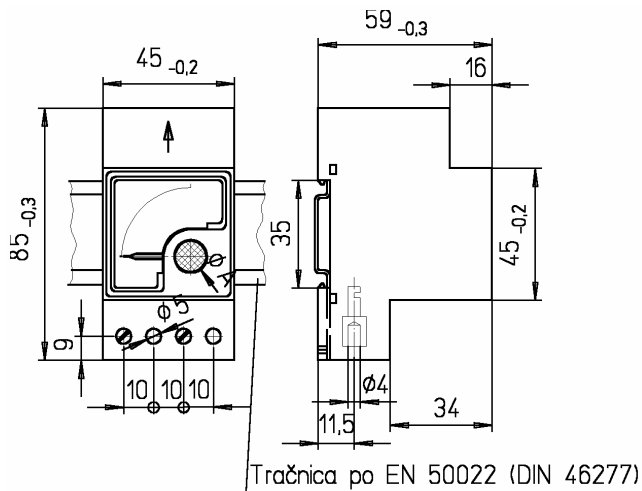
Picture 8: Dimensional drawing FQ0507 (all dimensions are in mm)
