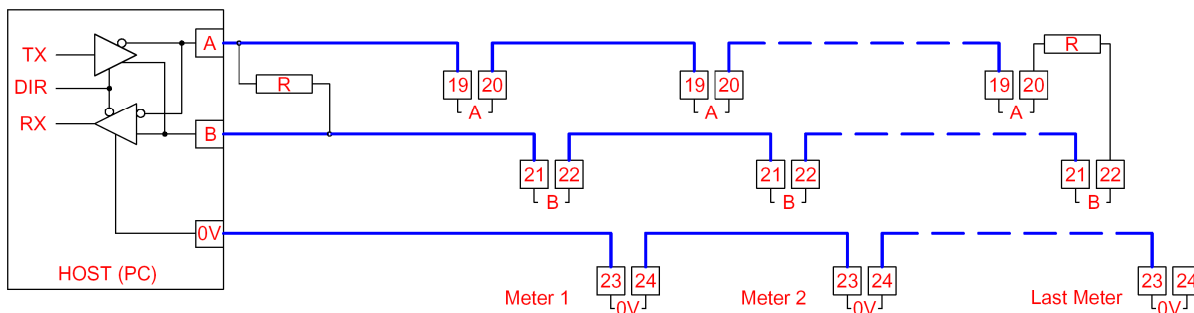
Figure 3-1 Basic RS485 Bus Network
